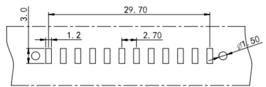
RECOMMENDED PCB LAYOUT T=0.65MM, TOLERANCES±0.05MM
